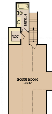
Bonus Room Floor Plan
